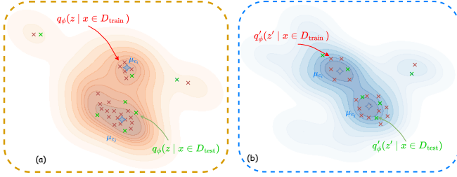
Fig. 2. Comparison of latent space distributions. (a) Original VAE latent space shows clear separation between training(Member) ( q_\phi(z|x \in D_{\text{train}}) ) and test(Non-member) samples ( q_\phi(z|x \in D_{\text{test}}) ). (b) Our privacy-enhanced VAE produces more dispersed latent distributions with increased overlap between training and test samples, making membership inference more difficult.
